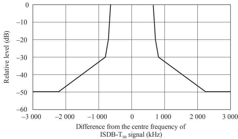
FIGURE 7 Spectrum mask for ISDB-T SB transmission signal (BW = 6/14 MHz, n = 3 )
