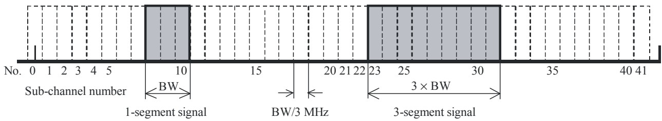
FIGURE 8 Definition of sub-channel
